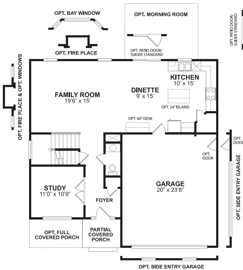
ELEVATION #1
