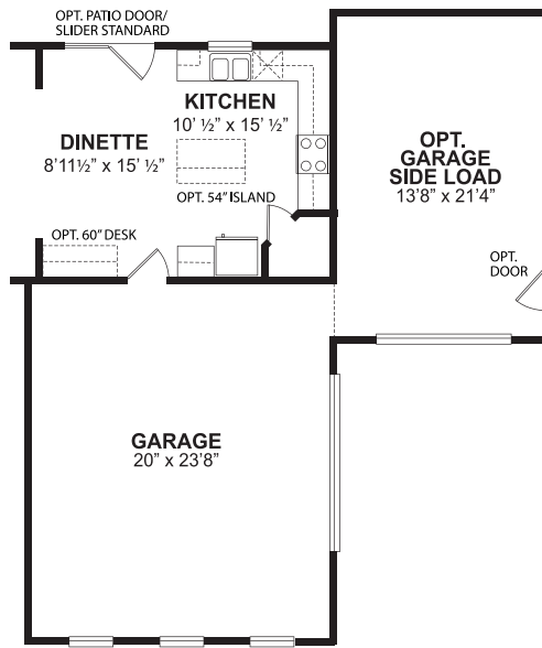
1ST FLOOR PLAN OPT. 3 CAR GARAGE PLANS
