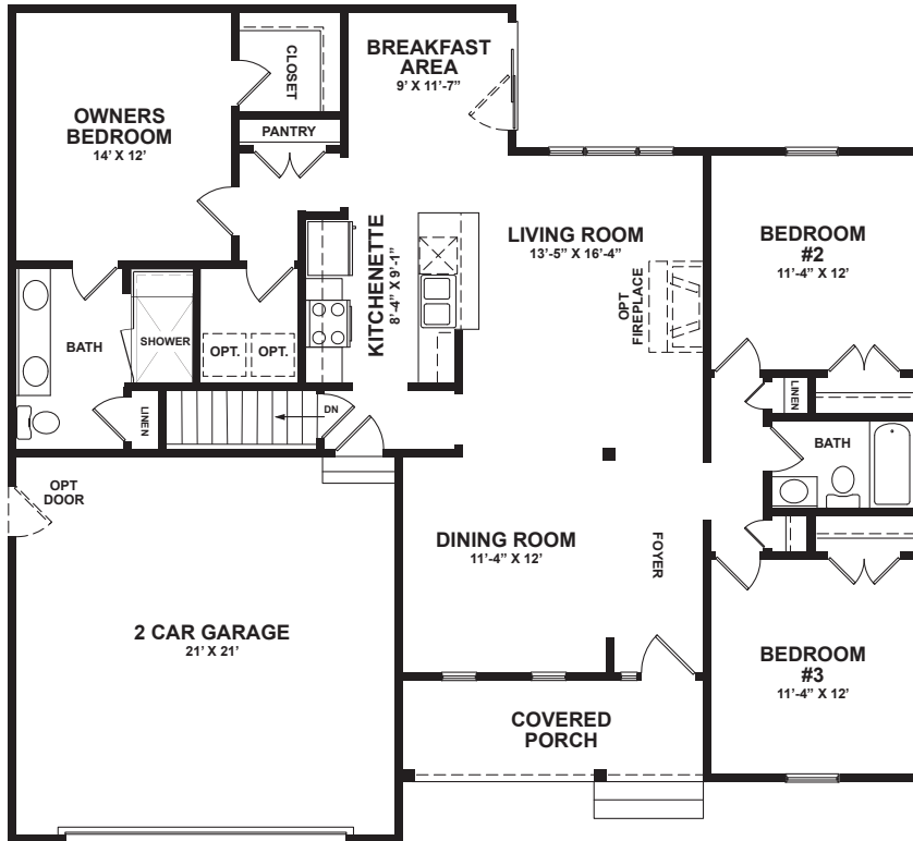
FIRST FLOOR
